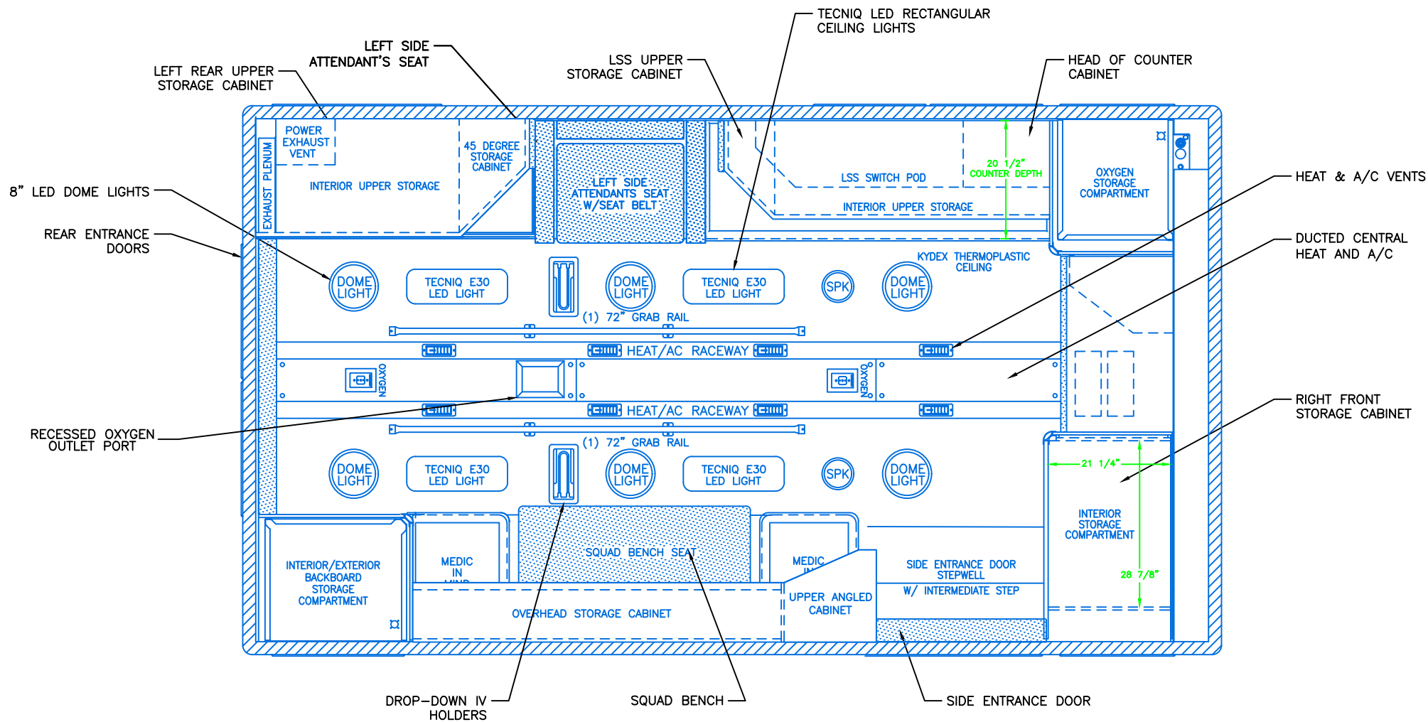
CEILING VIEW
