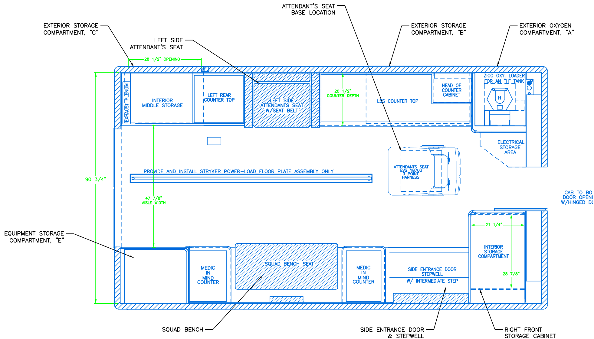
FLOOR PLAN
